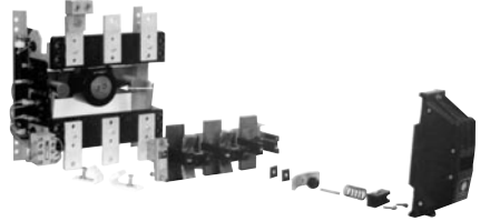
Typical NEMA Size 6 Contactor (exploded view)
